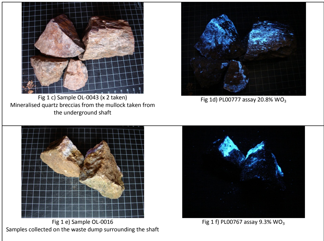
Figure 1: Figures (a-f) show samples taken with corresponding normal and then correspondingly under short wave ultraviolet light (UV). Sample numbers (a-b), (c-d) and (e-f) correspond to the same sample. Scheelite has a bright, pale blue iridescence under short wave ultraviolet light. 1cm squares for scale.
