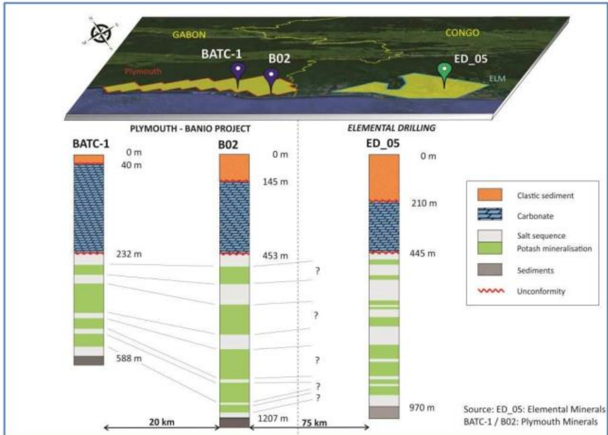
FIGURE 3: STRATIGRAPHIC SECTION SHOWING INTERPRETED CONTINUITY OF SALT SEQUENCES THROUGHOUT THE CONGO BASIN AS DEFINED BY DRILLING IN PLYMOUTH AND KORE POTASH TENURE
